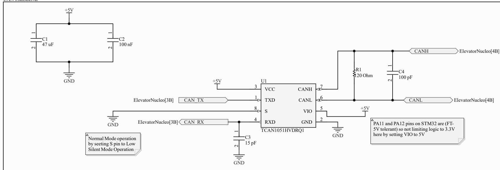
CAN Transceiver
