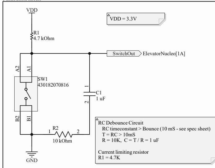
Pushbutton circuit
